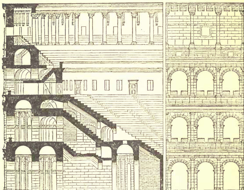
SECTION AND PORTION OF THE ELEVATION OF THE COLOSSEUM
